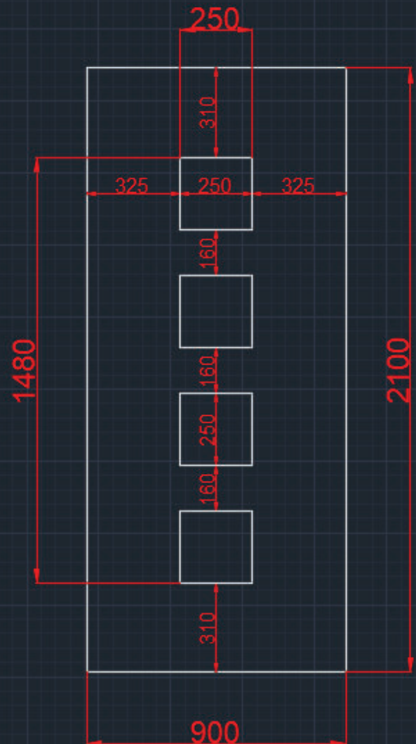
Technical Drawing (With Dimensions) (mm)
