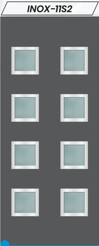
Panel Dimension: 900x2000 (Other lenght upon request) Colour : RAL 7016 Design : 500x1540
