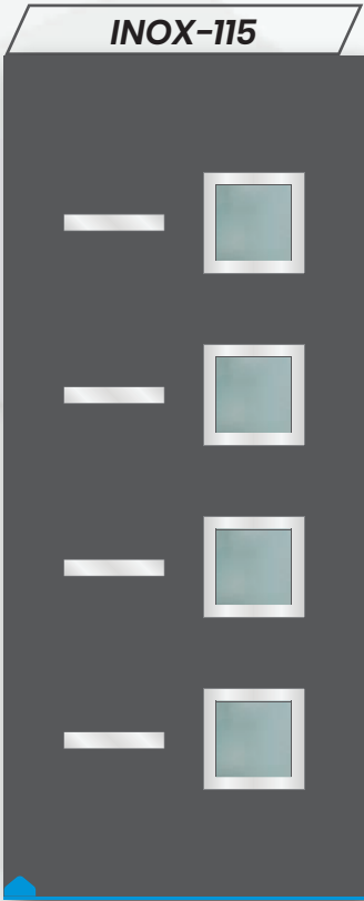
Panel Dimension: 900x2000 (Other lenght upon request) Colour : RAL 7016 Design : 600x1540
