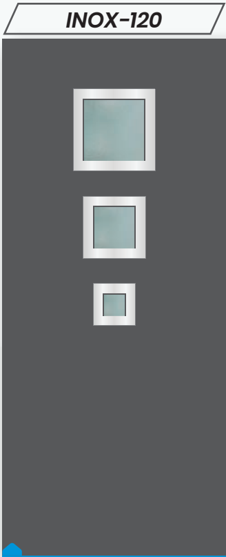
Panel Dimension: 900x2000 (Other lenght upon request) Colour : RAL 7016 Design : 330x950
