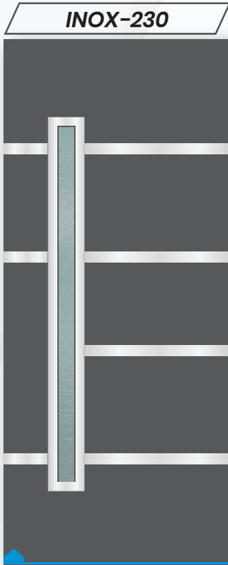
Panel Dimension: 900x2000 (Other lenght upon request) Colour : RAL 7016 Design : 888x1480
